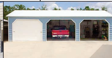
30' x 51' x 12' - 12 Gauge Vertical Roof 12X12 Roll up, 10X10 Roll up 36" Walk door, 4 window
